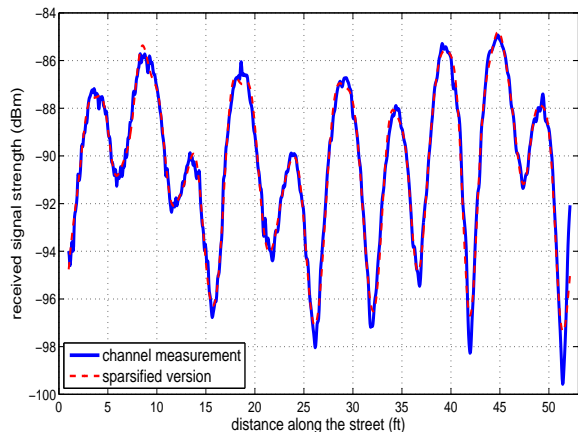
Fig. 2. Channel measurement along a street in San Francisco (courtesy of Mark Smith [48]) and its sparsified version. The two curves are almost identical.
