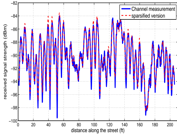
Fig. 4. Another channel measurement along a street in San Francisco (courtesy of Mark Smith [48]) and its sparsified version. The two curves are almost identical.
