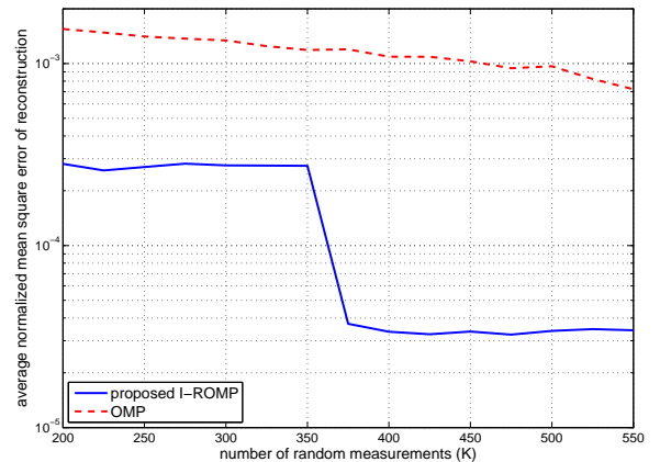
Fig. 7. Reconstruction of the measured channel of Fig. 4 based on an incomplete observation set using compressed sensing (length of X is N = 4096 ). The ROMP result is excluded as its error is significantly higher than the rest.
