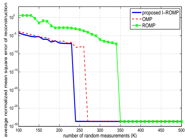
Fig. 3. Reconstruction of the sparsified signal of Fig. 2 based on an incomplete observation set using compressed sensing (length of X is N = 1024 ).
