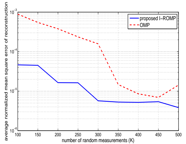
Fig. 6. Reconstruction of the measured channel of Fig. 2 based on an incomplete observation set using compressed sensing (length of X is N = 1024 ). The ROMP result is excluded as its error is significantly higher than the rest.
